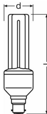
DSST STICK 23 W/825 B22D
