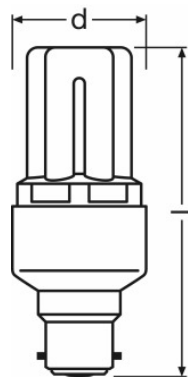
DSST STICK 8 W/825 B22D
