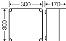
Dimension drawing
